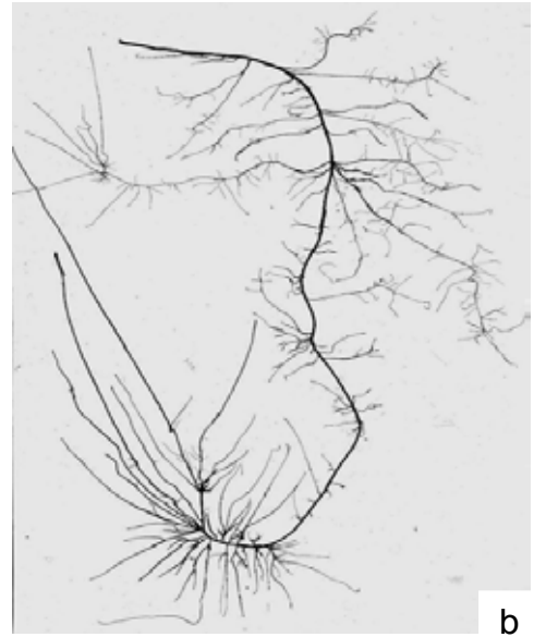
Figure 2 Individual roots of perennial ryegrass cv. 'Alto': (a) from position or phytomer eight (the 3 rd root-bearing phytomer) and (b) from phytomer 12 (four leaf appearance intervals older) of the same plant genotype in Experiment 1; (c) from phytomer 12 of a genotype in Experiment 1 identified by principal component analysis (see text) as having differing morphology from (b); (d) from phytomer 16 in Experiment 2 (autumn), with roots of similar age to phytomer 12 in Experiment 1.
