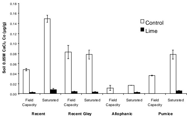
Figure 5 Effect of lime, soil moisture status and soil groups on 0.05M CaCl 2 extractable Co measured after harvest in Pot Trial 2.
