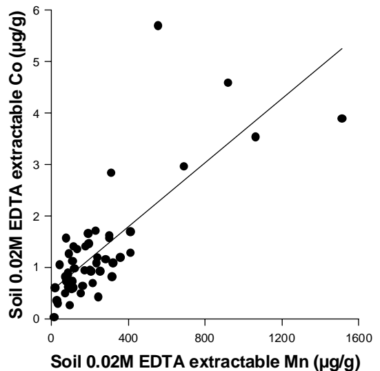
Figure 1 The relationship between soil 0.02M EDTA Co and 0.02M EDTA Mn in 51 topsoils.
