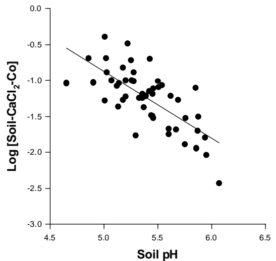
Figure 2 The relationship between soil pH and soil 0.05M CaCl 2 Co in 51 topsoils.
