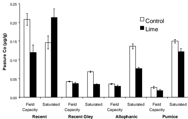
Figure 4 Effect of lime, soil moisture status and soil groups on pasture Co in Pot Trial 2.
