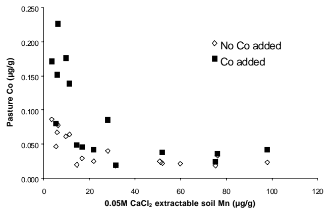
Figure 3 Effect of added Co fertiliser and soil Mn status, measured by 0.05M CaCl 2 extract, on pasture Co levels in Pot Trial 1.
